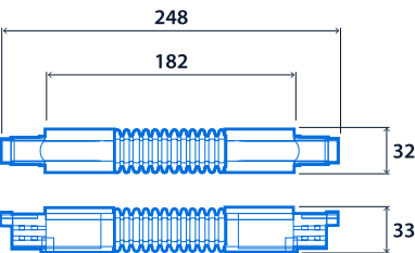
Flexible Coupler
