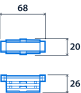
Straight Coupler
