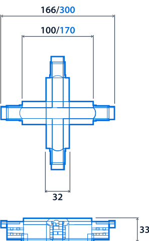
Cross feed
