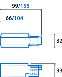
Feed
