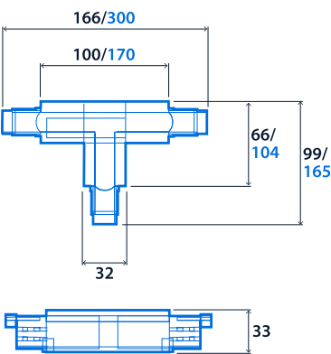
Tee Feed/Coupler
