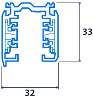
3-Circuit Track
