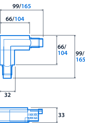
Angled Feed/Coupler
