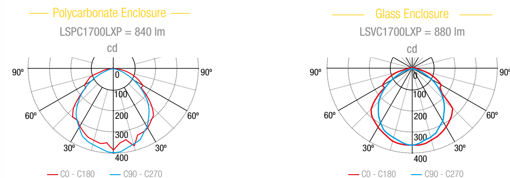
PHOTOMETRIC GUIDE
