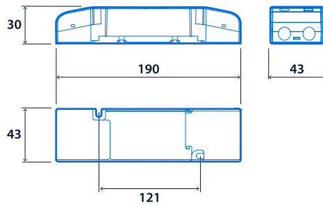
DALI Remote Driver
