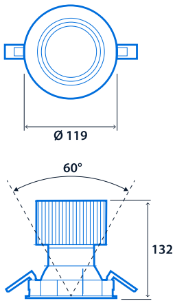
Cut-out - Ø 110 Minimum ceiling void - 180
