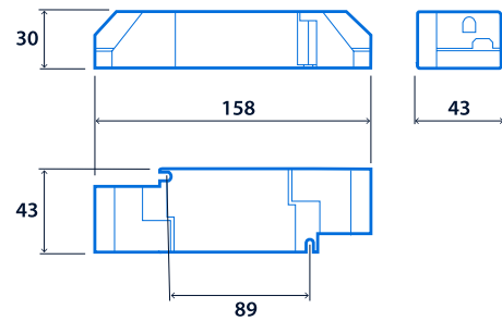
Non-Dimming Remote Driver
