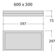
Cut out for plasterboard ceiling type: 576 X 276
