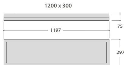
Cut out for plasterboard ceiling type: 1176 X 276
