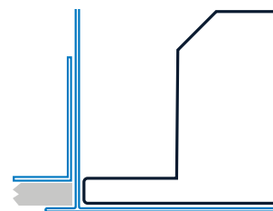
Plasterboard ceiling with recessing frame
