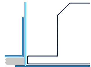
Plasterboard ceiling with recessing frame
