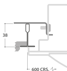
Exposed T-bar (15mm or 24mm)
