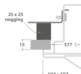
Plasterboard Ceiling
