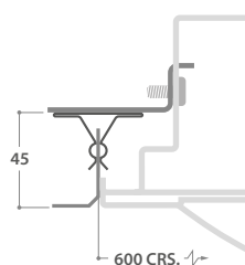
Spring Tee
