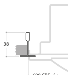
Lay-in on Exposed T-bar (15mm or 24mm)
