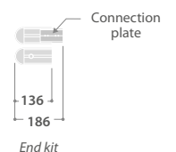
End kit
