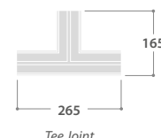
Tee Joint
