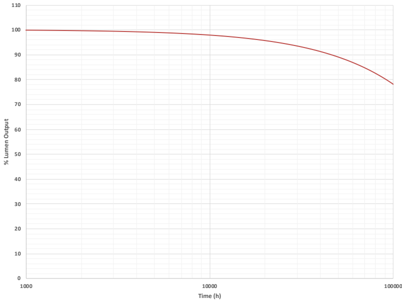
LUMEN DEPRECIATION CURVE
