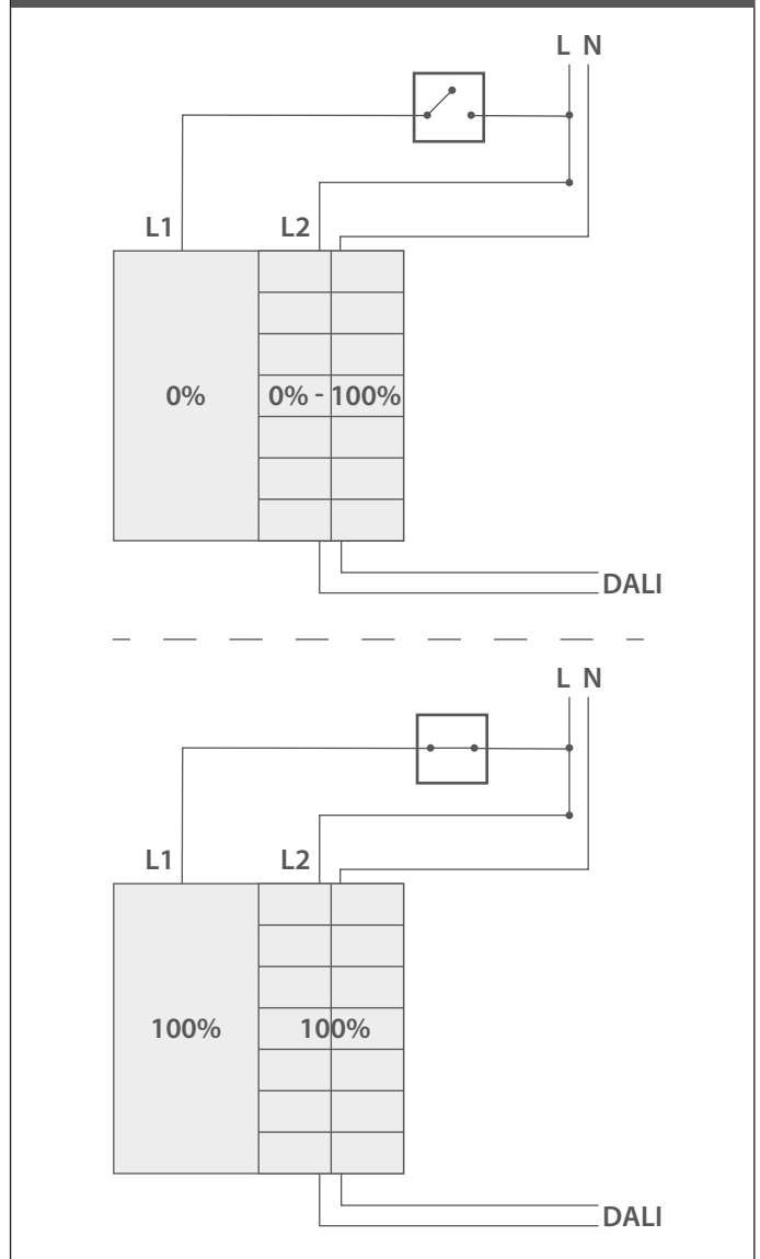
5b. SCHEMATIC
