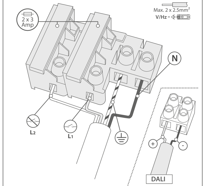
5b. SCHEMATIC
