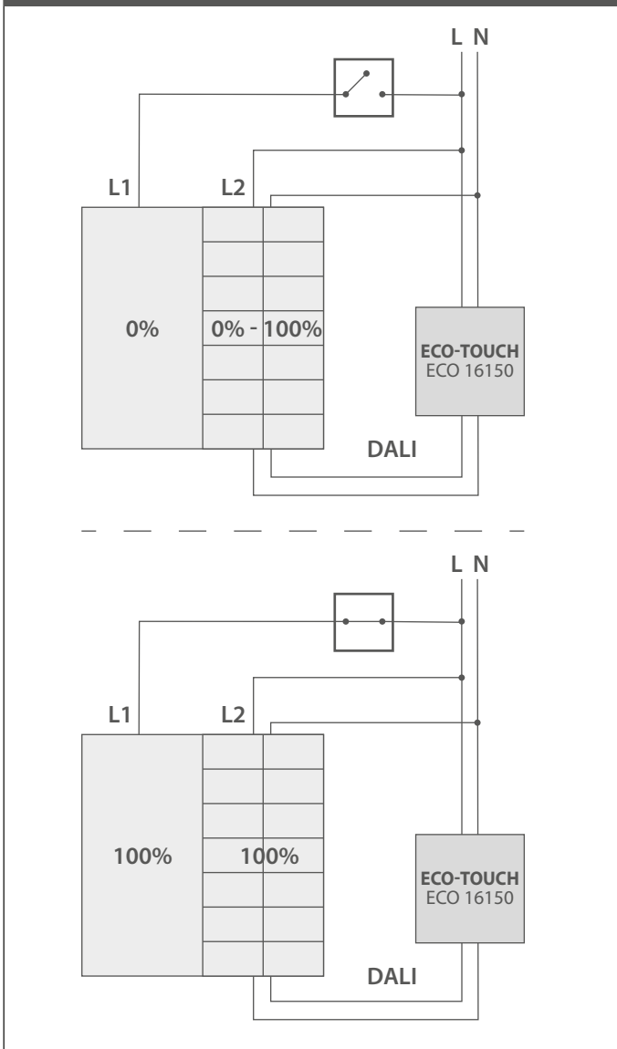
5a. SCHEMATIC WITH ECO 16150
