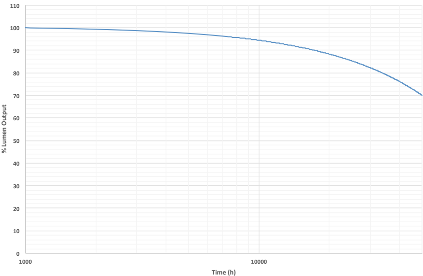
LUMEN DEPRECIATION CURVE
