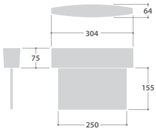
Ceiling Mounting
