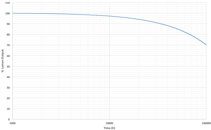
LUMEN DEPRECIATION CURVE
