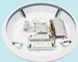
Dot retrofit LED gear tray
